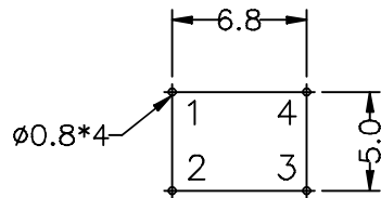
SUGGESTED P.C.B LAYOUT
